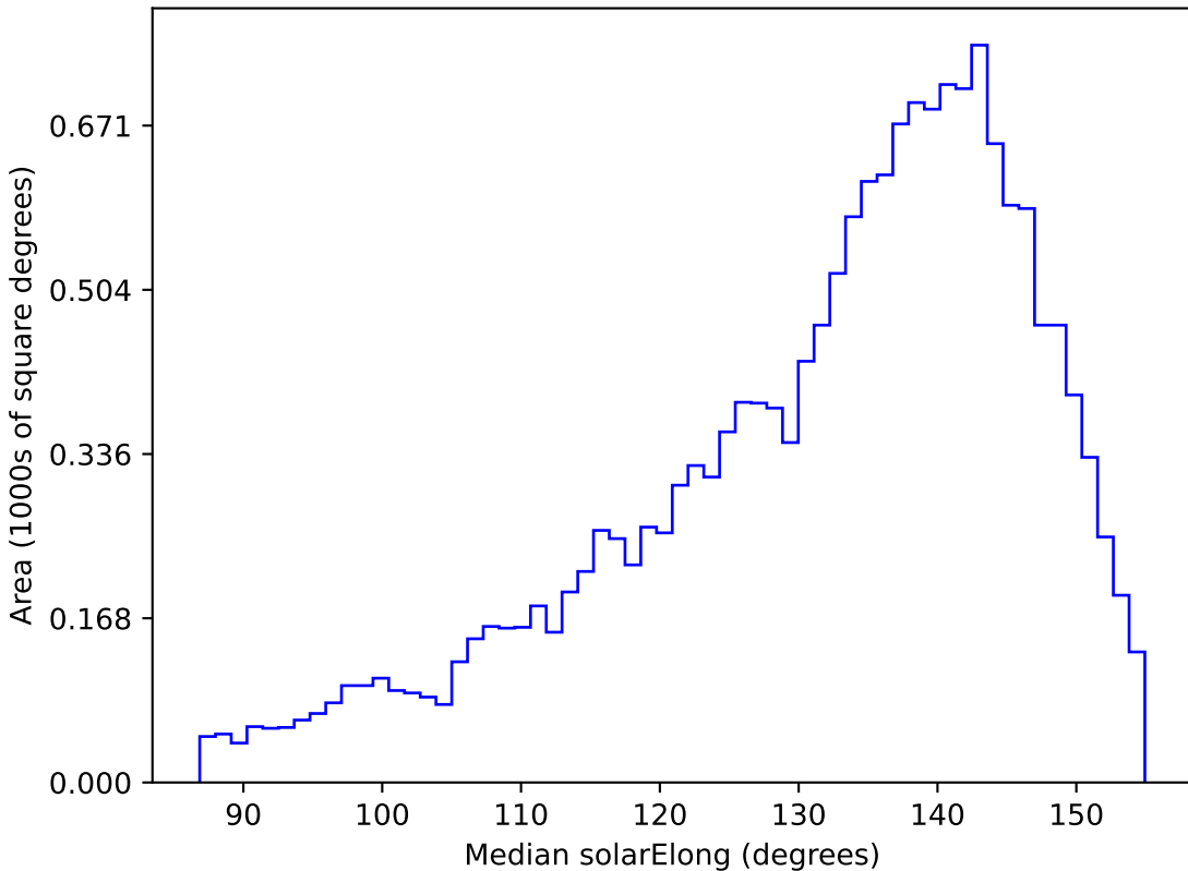
extra_ss_neo3_v3.4_10yrs WFD u band: Median solarElong
