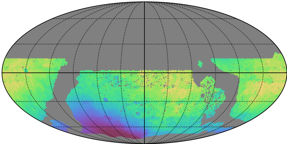
extra_ss_neo3_v3.4_10yrs WFD i band: Median solarElong
