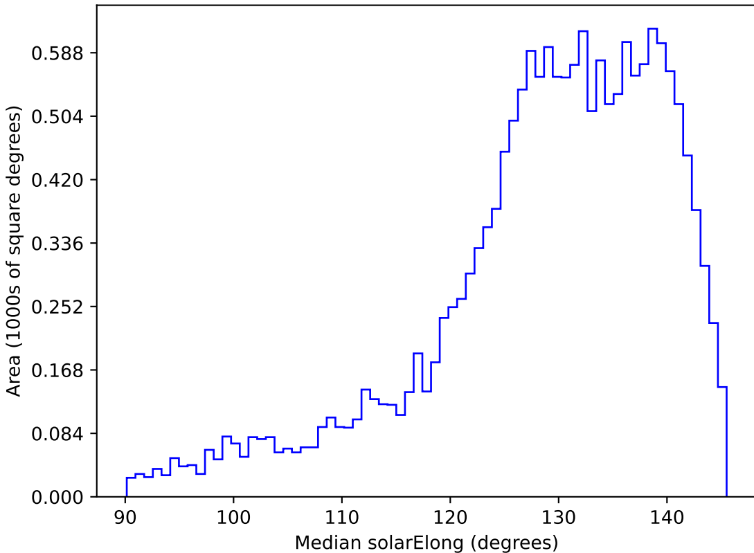
extra_ss_neo3_v3.4_10yrs WFD i band: Median solarElong
