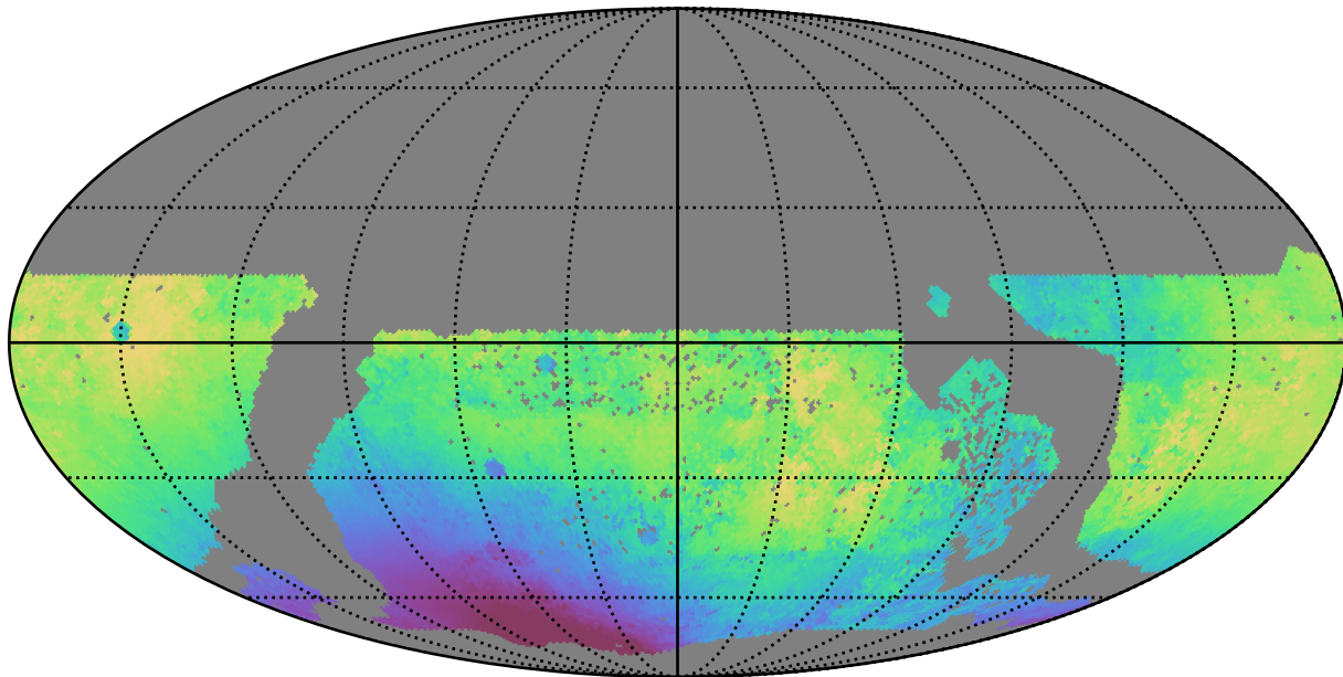
extra_ss_neo3_v3.4_10yrs WFD g band: Median solarElong
