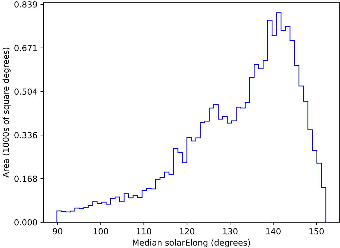
extra_ss_neo3_v3.4_10yrs WFD g band: Median solarElong
