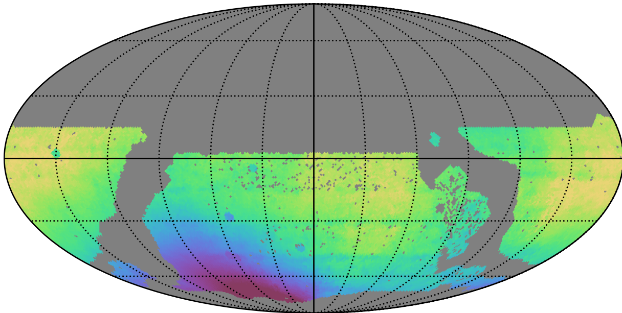
extra_ss_neo3_v3.4_10yrs WFD all bands: Median solarElong
