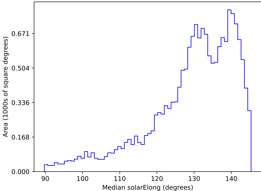
extra_ss_neo3_v3.4_10yrs WFD all bands: Median solarElong
