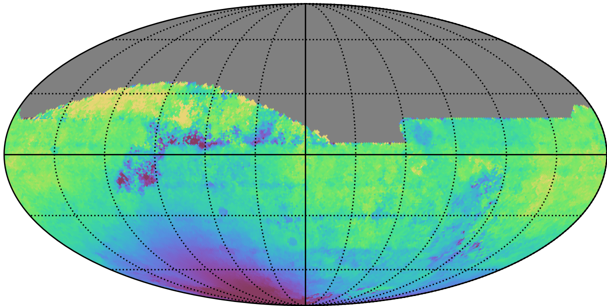
extra_ss_neo3_v3.4_10yrs All sky z band: Median solarElong
