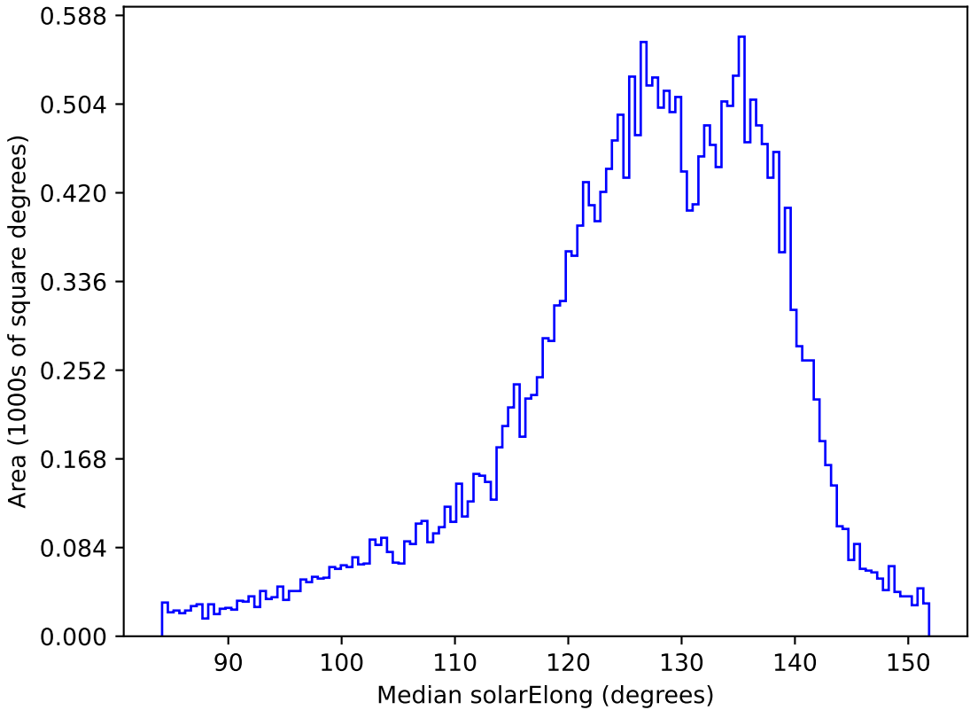
extra_ss_neo3_v3.4_10yrs All sky z band: Median solarElong
