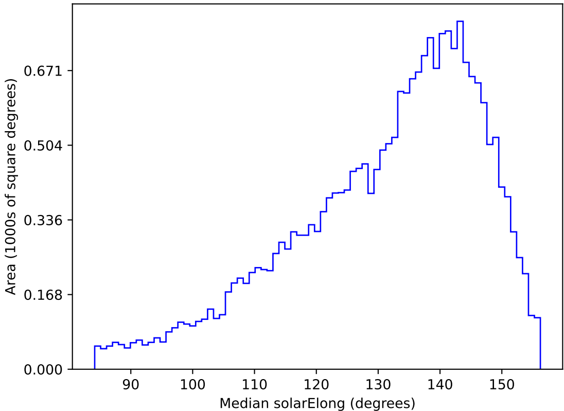
extra_ss_neo3_v3.4_10yrs All sky u band: Median solarElong
