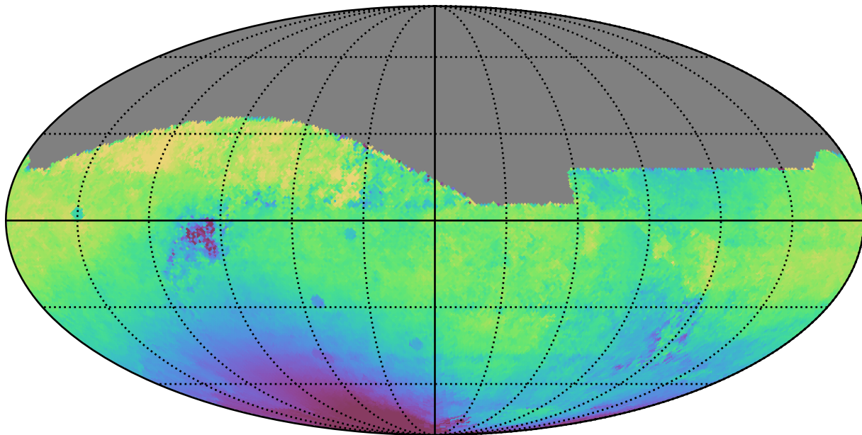
extra_ss_neo3_v3.4_10yrs All sky r band: Median solarElong
