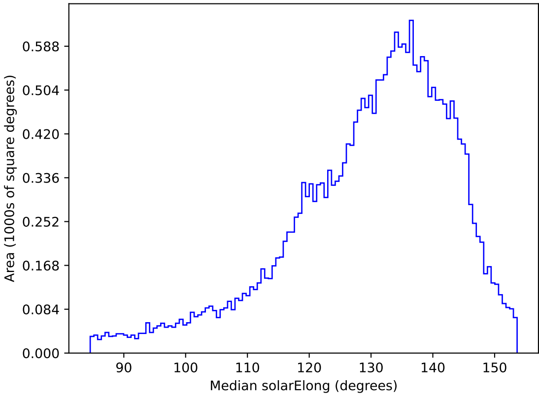
extra_ss_neo3_v3.4_10yrs All sky r band: Median solarElong
