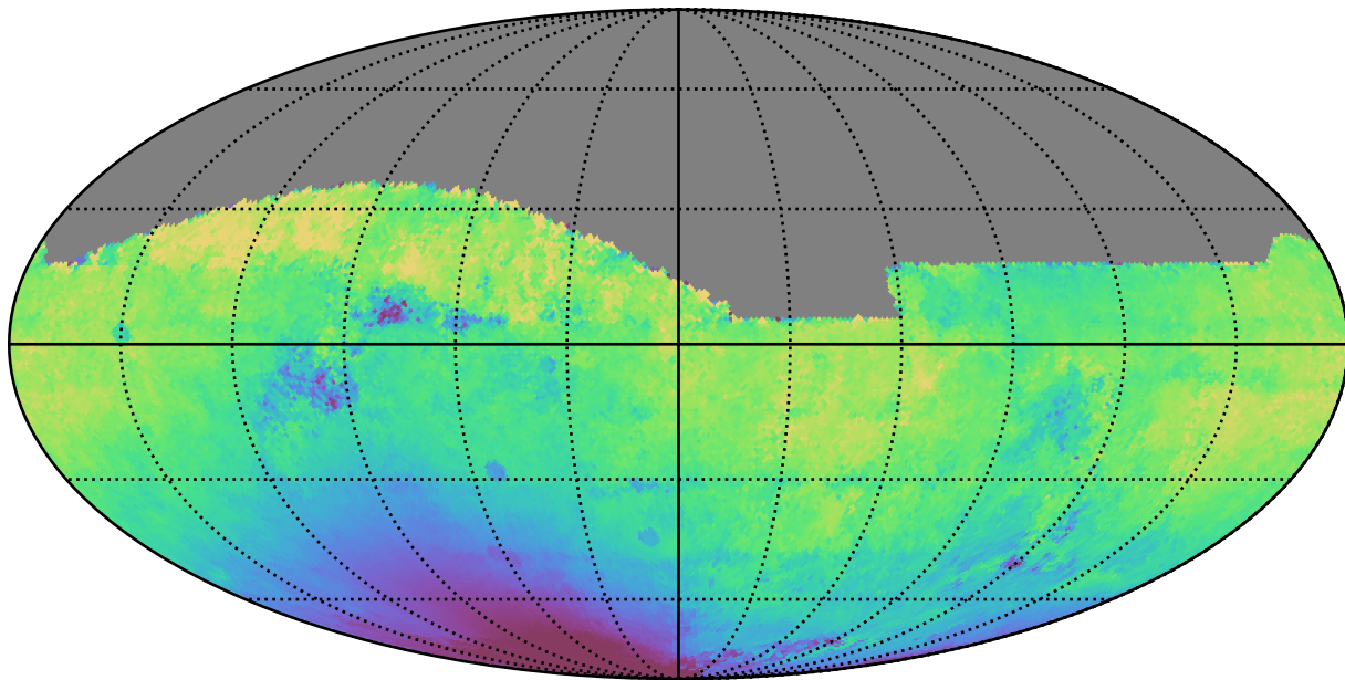
extra_ss_neo3_v3.4_10yrs All sky i band: Median solarElong
