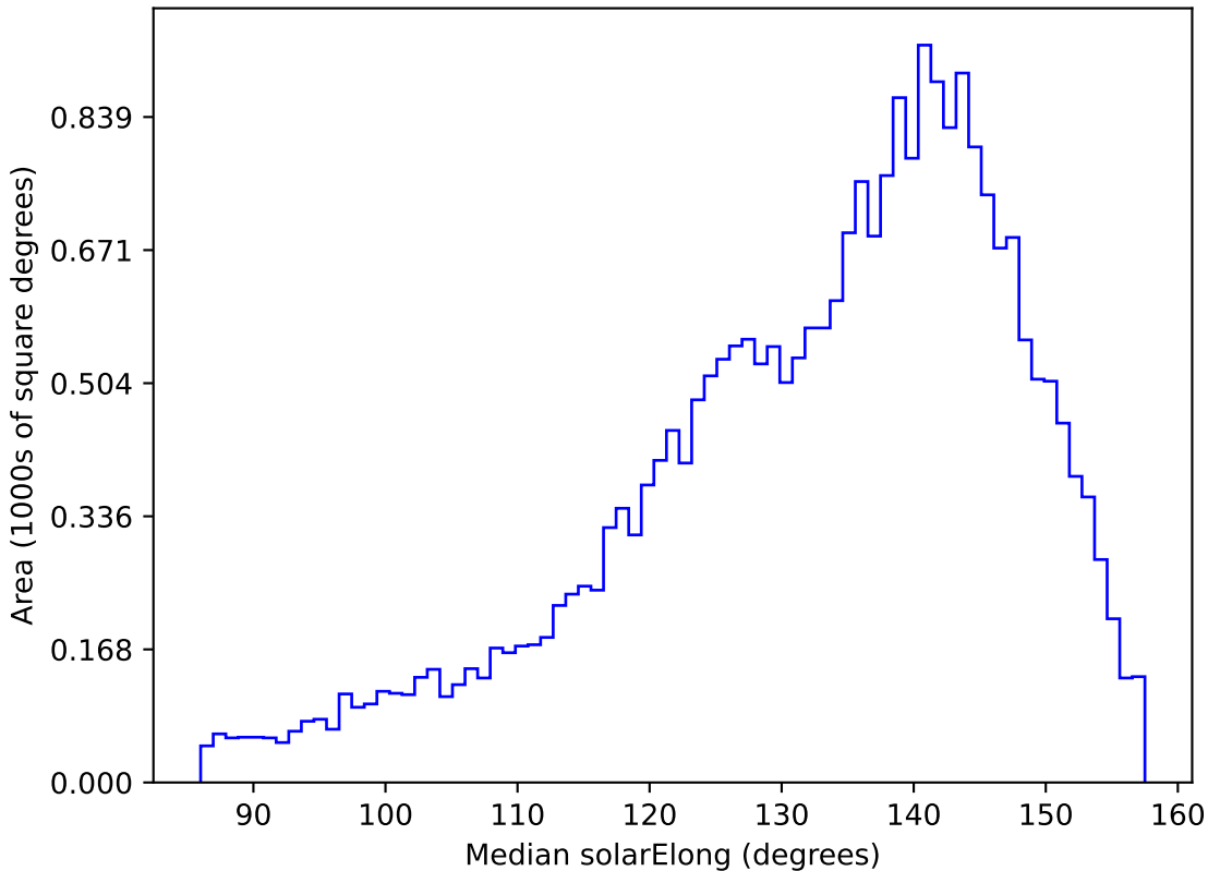
extra_ss_neo3_v3.4_10yrs All sky g band: Median solarElong
