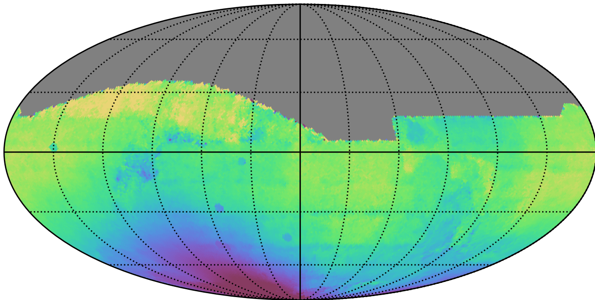
extra_ss_neo3_v3.4_10yrs All sky all bands: Median solarElong
