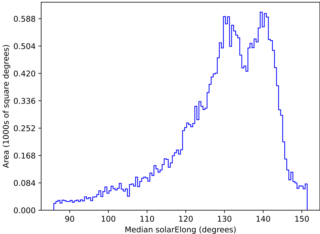
extra_ss_neo3_v3.4_10yrs All sky all bands: Median solarElong
