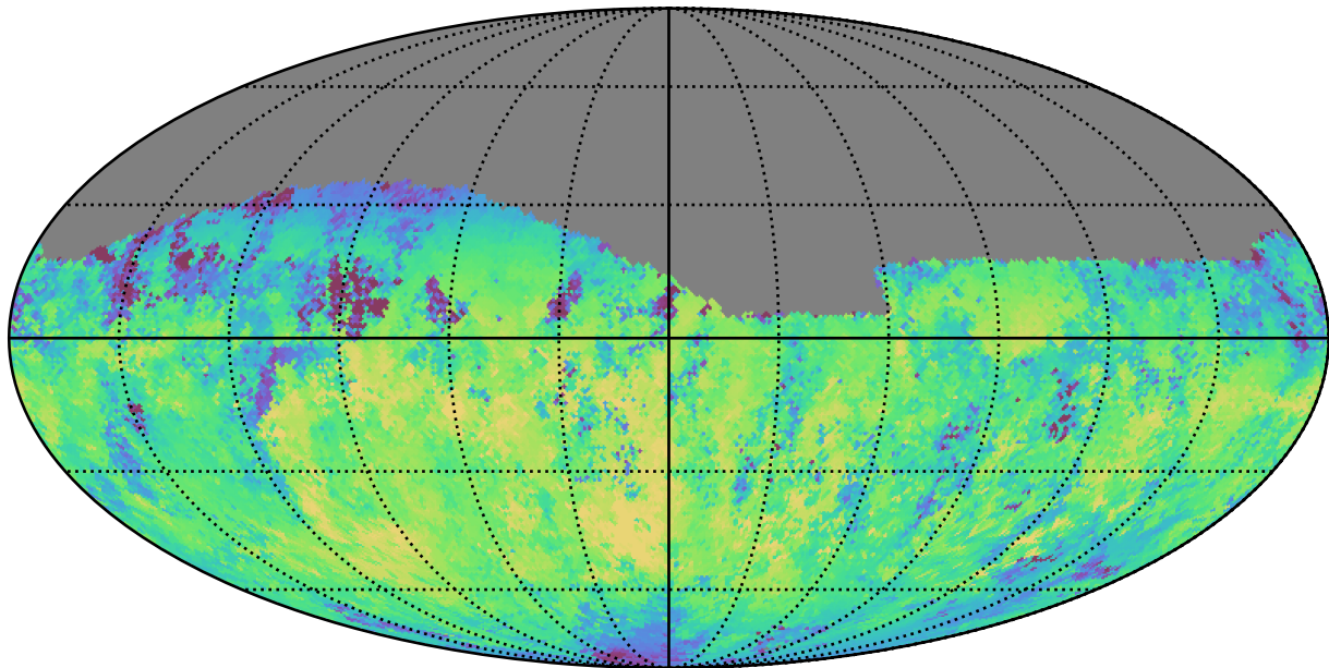
extra_ss_neo3_v3.4_10yrs Yr 1 z band: Median skyBrightness
