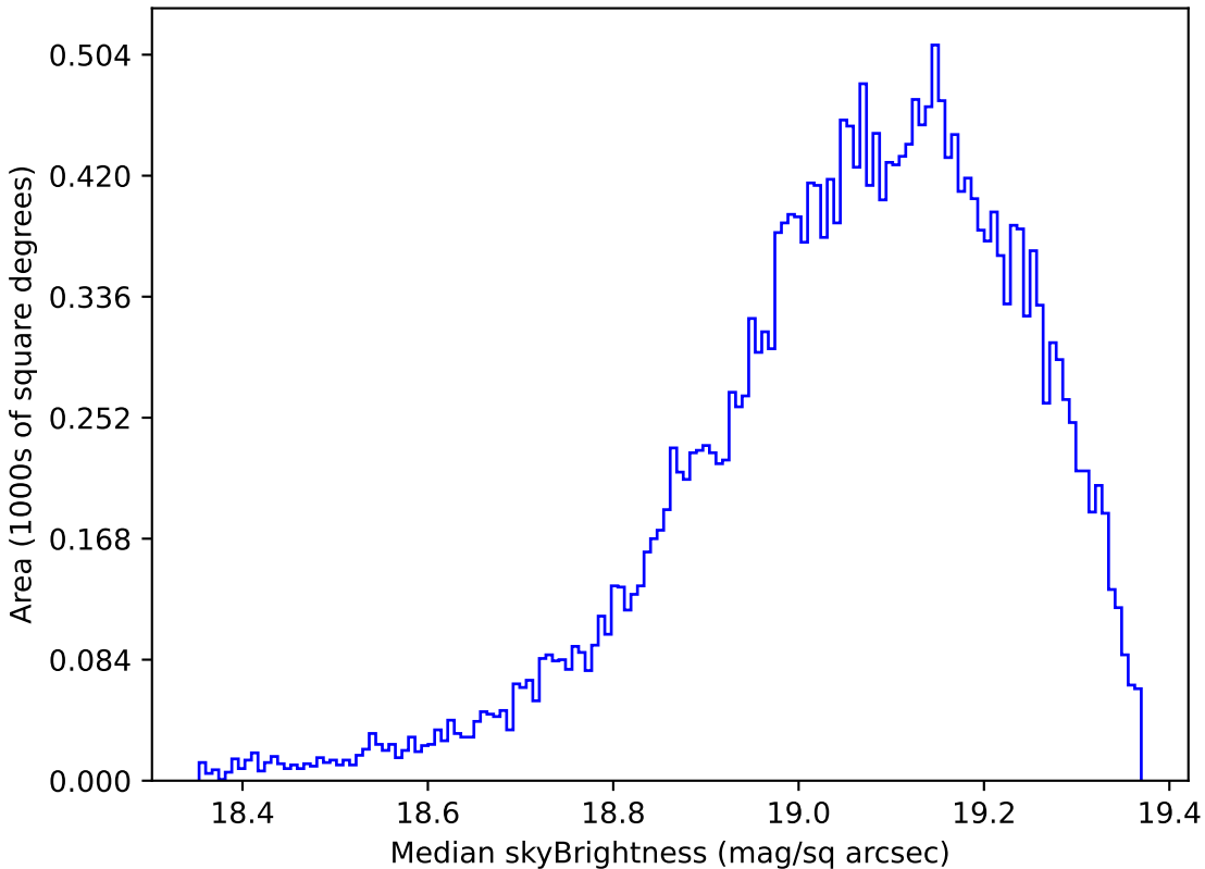
extra_ss_neo3_v3.4_10yrs Yr 1 z band: Median skyBrightness
