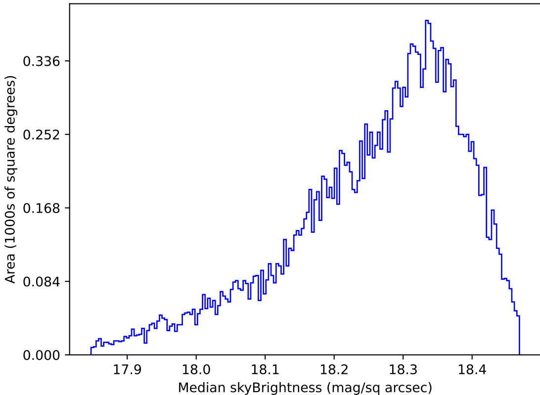
extra_ss_neo3_v3.4_10yrs Yr 1 y band: Median skyBrightness
