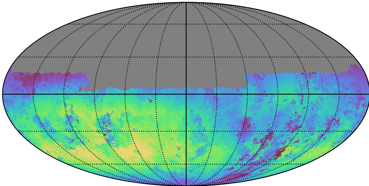
extra_ss_neo3_v3.4_10yrs Yr 1 u band: Median skyBrightness
