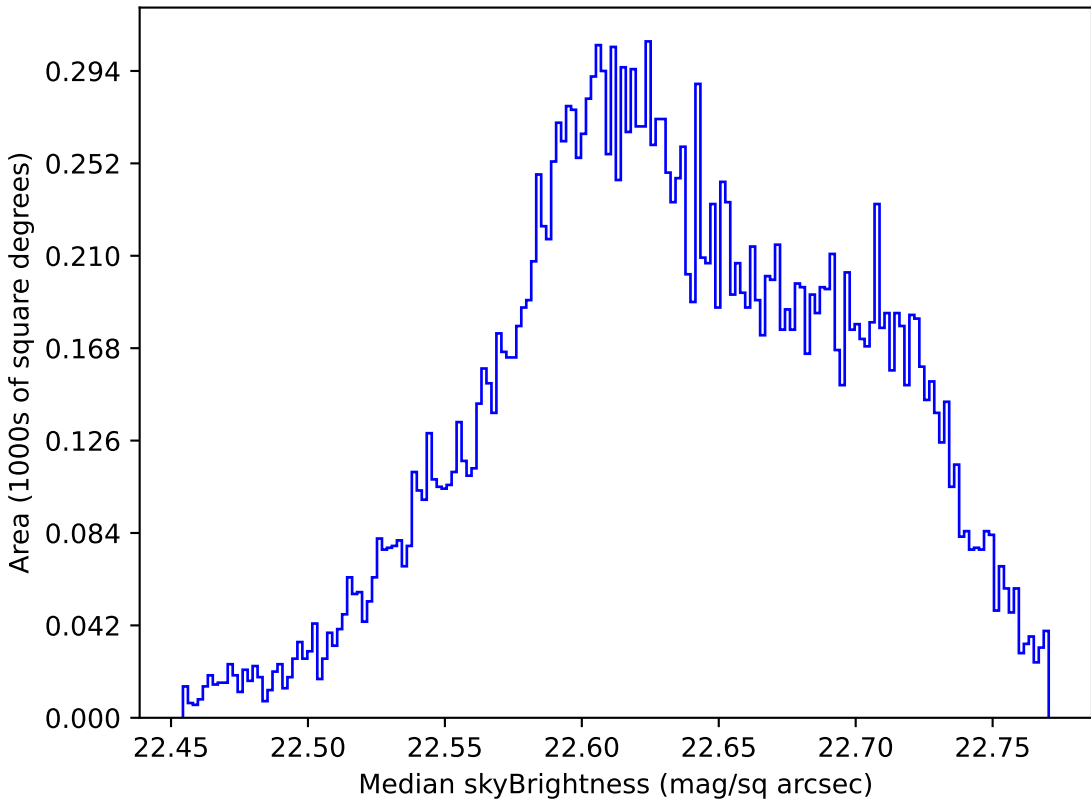
extra_ss_neo3_v3.4_10yrs Yr 1 u band: Median skyBrightness
