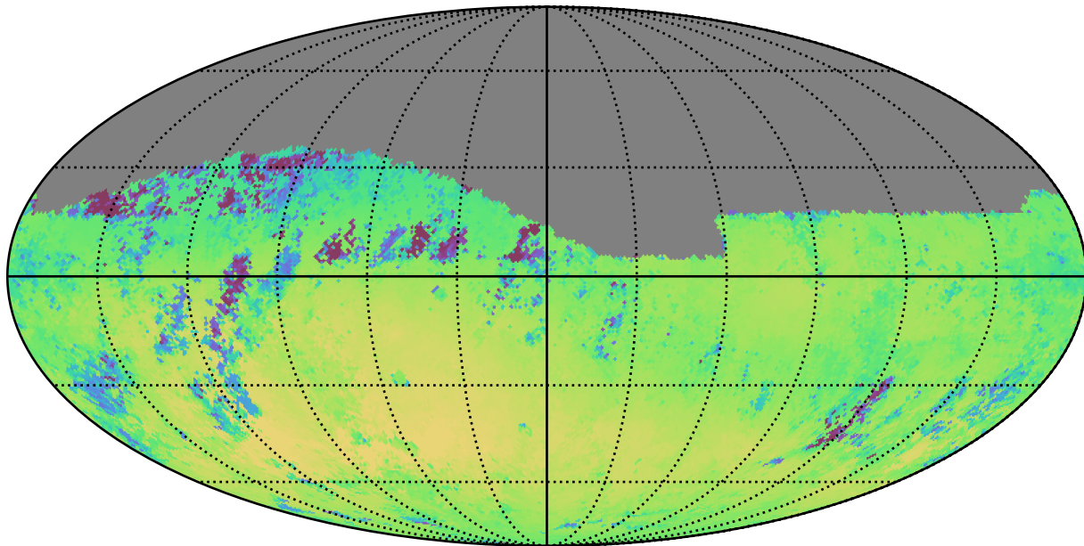
extra_ss_neo3_v3.4_10yrs Yr 1 r band: Median skyBrightness
