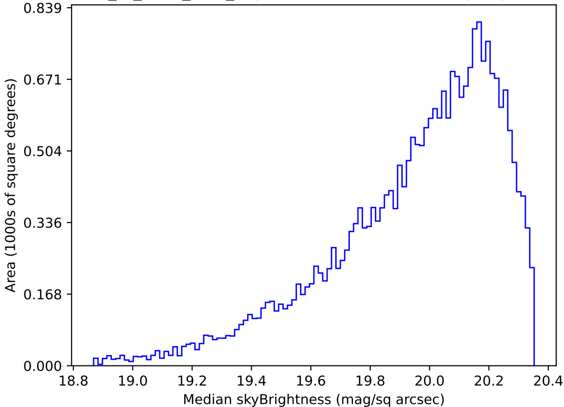
extra_ss_neo3_v3.4_10yrs Yr 1 i band: Median skyBrightness
