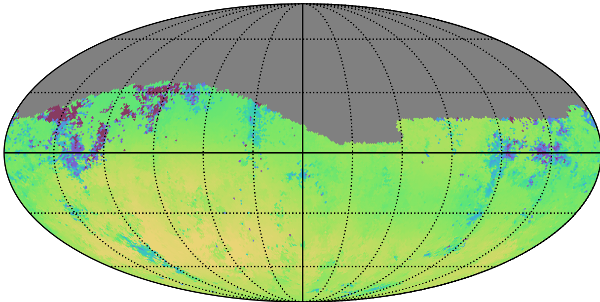
extra_ss_neo3_v3.4_10yrs Yr 1 g band: Median skyBrightness
