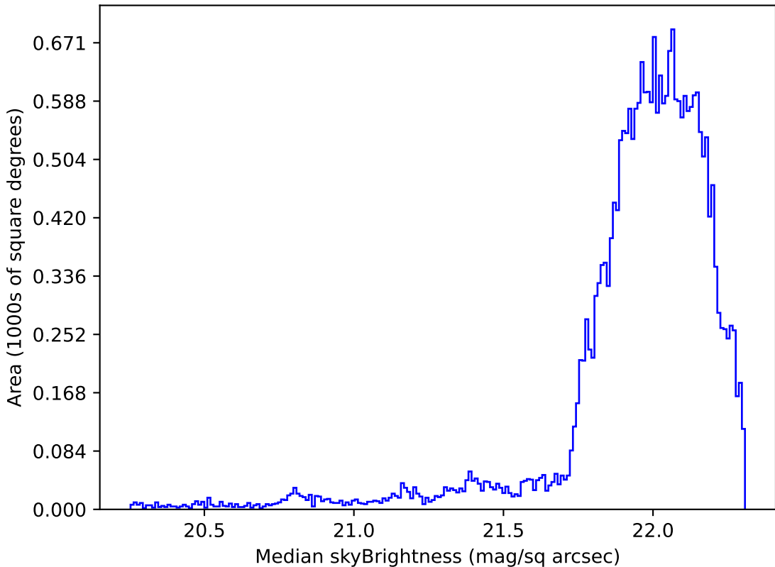
extra_ss_neo3_v3.4_10yrs Yr 1 g band: Median skyBrightness
