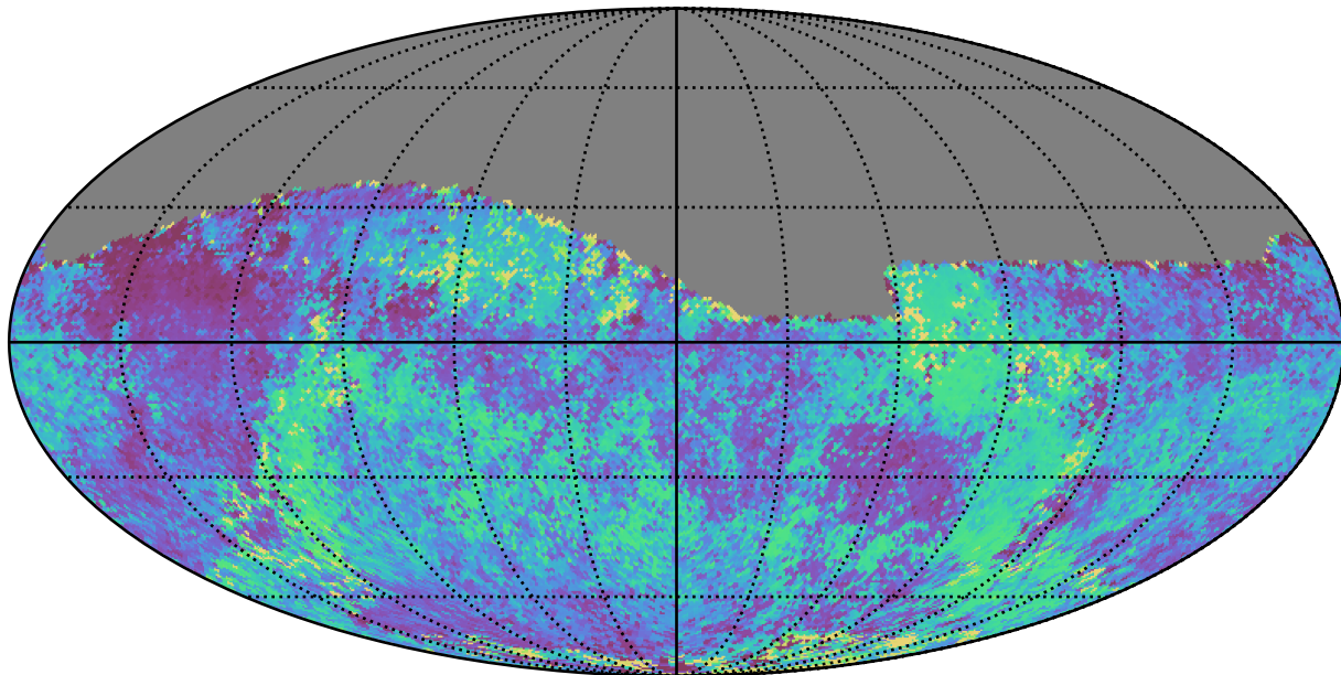
extra_ss_neo3_v3.4_10yrs Yr 1 all bands: Median skyBrightness
