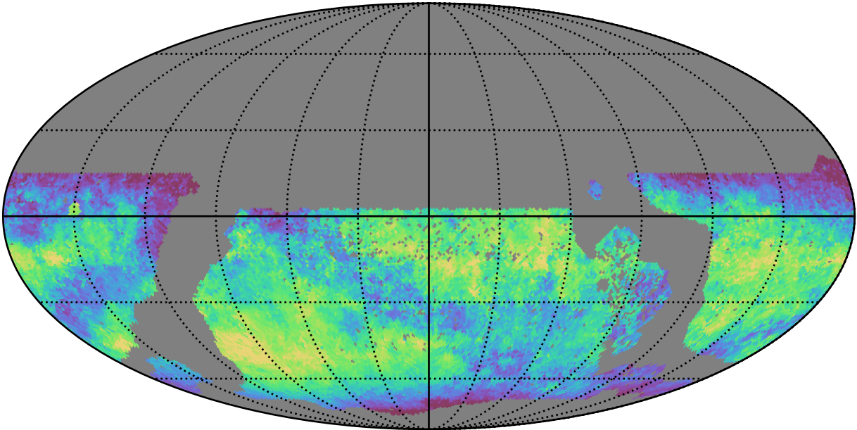
extra_ss_neo3_v3.4_10yrs WFD z band: Median skyBrightness
