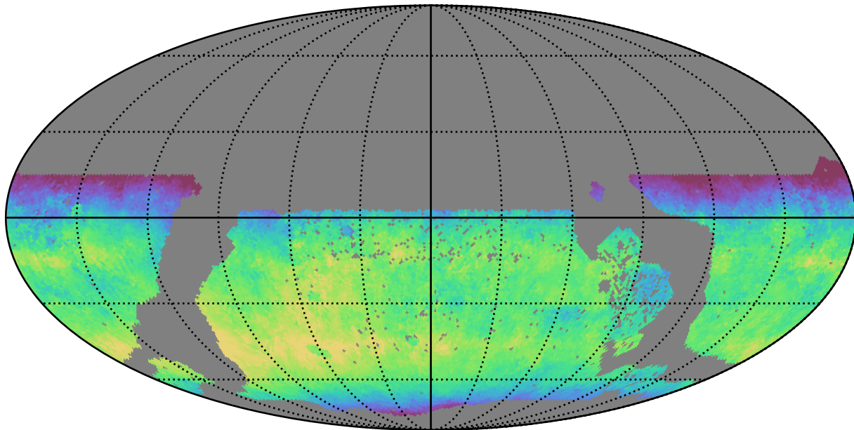
extra_ss_neo3_v3.4_10yrs WFD y band: Median skyBrightness
