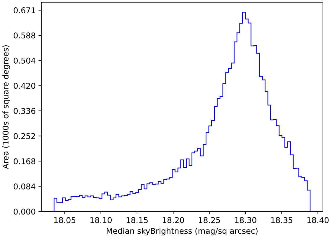
extra_ss_neo3_v3.4_10yrs WFD y band: Median skyBrightness
