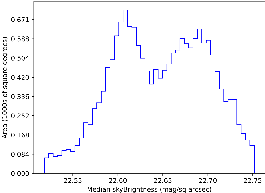
extra_ss_neo3_v3.4_10yrs WFD u band: Median skyBrightness
