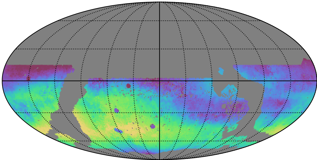
extra_ss_neo3_v3.4_10yrs WFD r band: Median skyBrightness
