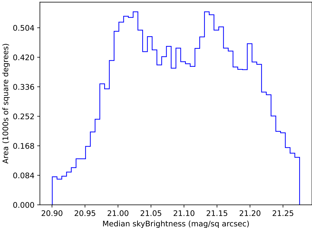
extra_ss_neo3_v3.4_10yrs WFD r band: Median skyBrightness
