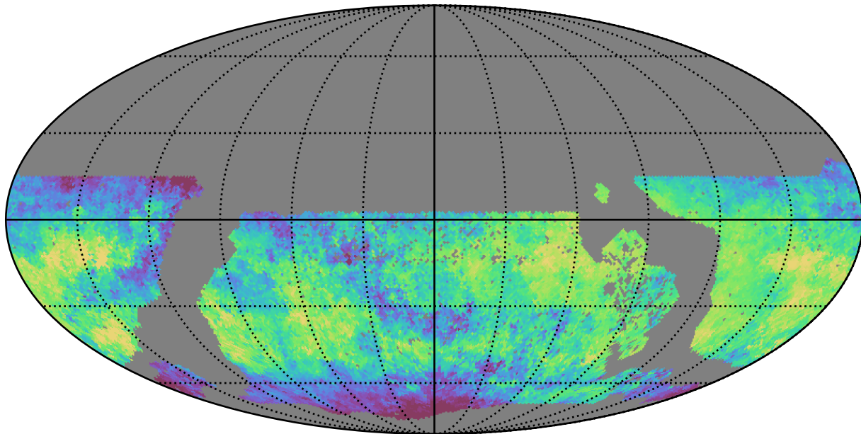
extra_ss_neo3_v3.4_10yrs WFD i band: Median skyBrightness
