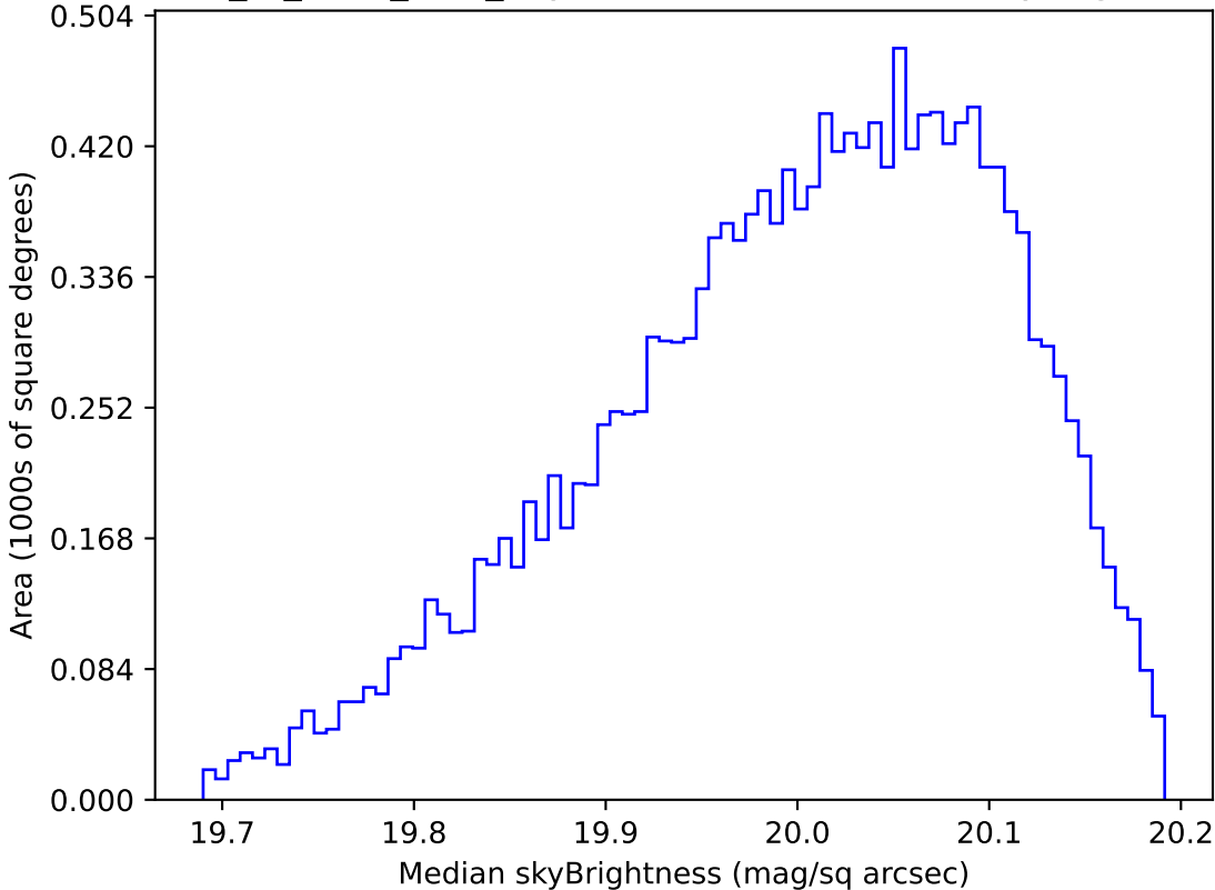
extra_ss_neo3_v3.4_10yrs WFD i band: Median skyBrightness
