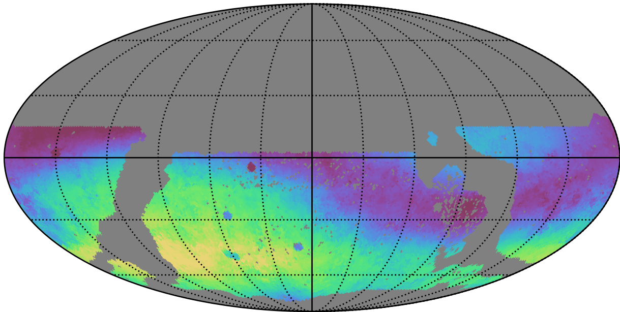
extra_ss_neo3_v3.4_10yrs WFD g band: Median skyBrightness
