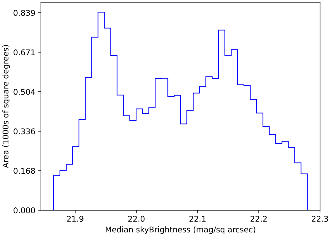
extra_ss_neo3_v3.4_10yrs WFD g band: Median skyBrightness
