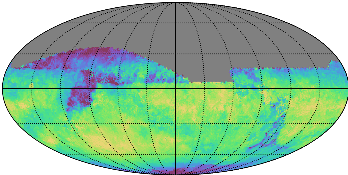
extra_ss_neo3_v3.4_10yrs All sky z band: Median skyBrightness
