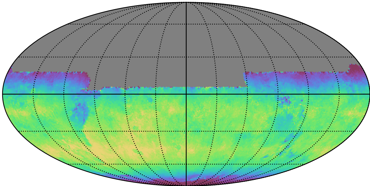
extra_ss_neo3_v3.4_10yrs All sky y band: Median skyBrightness
