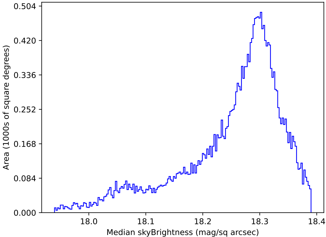
extra_ss_neo3_v3.4_10yrs All sky y band: Median skyBrightness
