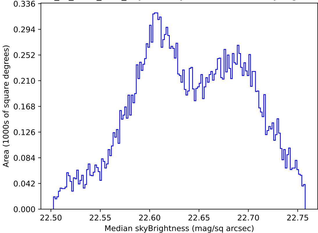
extra_ss_neo3_v3.4_10yrs All sky u band: Median skyBrightness
