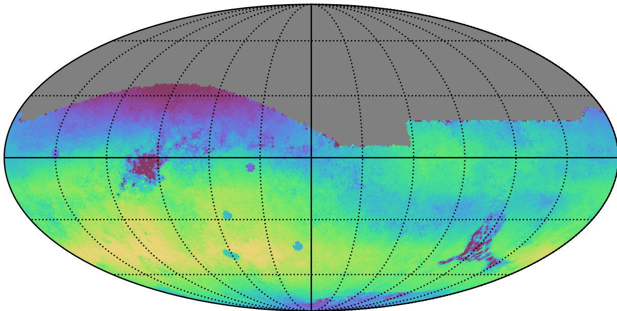
extra_ss_neo3_v3.4_10yrs All sky r band: Median skyBrightness
