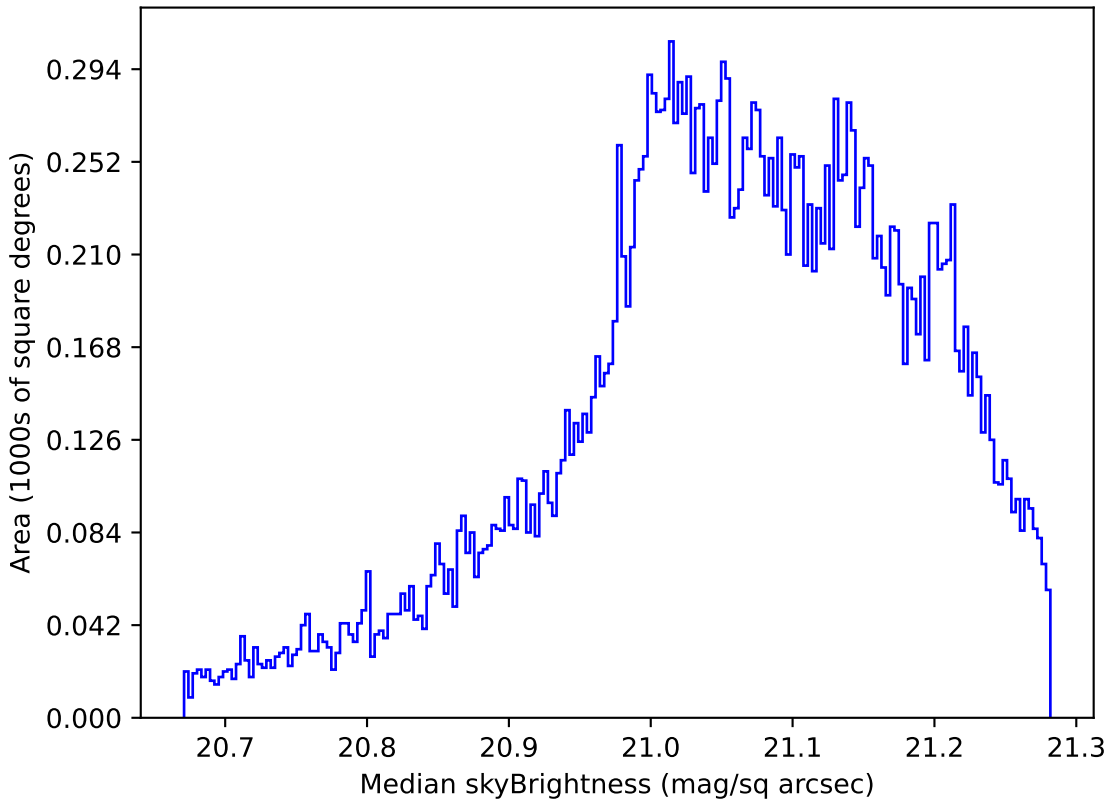
extra_ss_neo3_v3.4_10yrs All sky r band: Median skyBrightness
