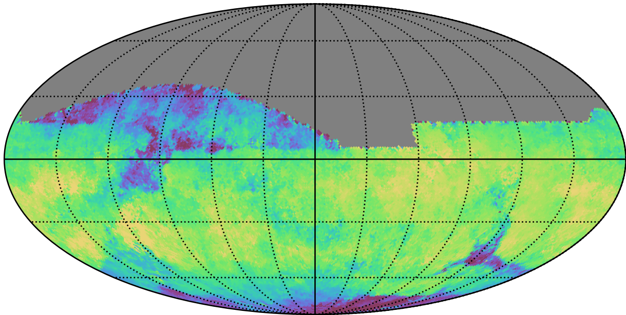
extra_ss_neo3_v3.4_10yrs All sky i band: Median skyBrightness
