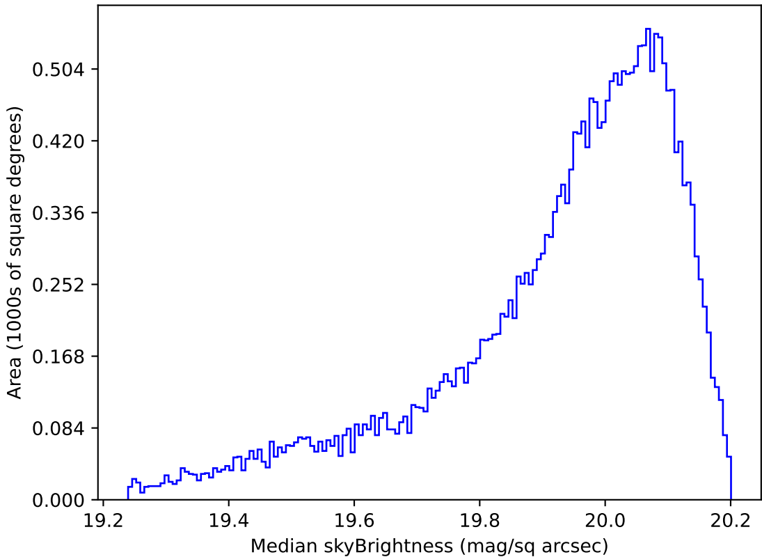
extra_ss_neo3_v3.4_10yrs All sky i band: Median skyBrightness
