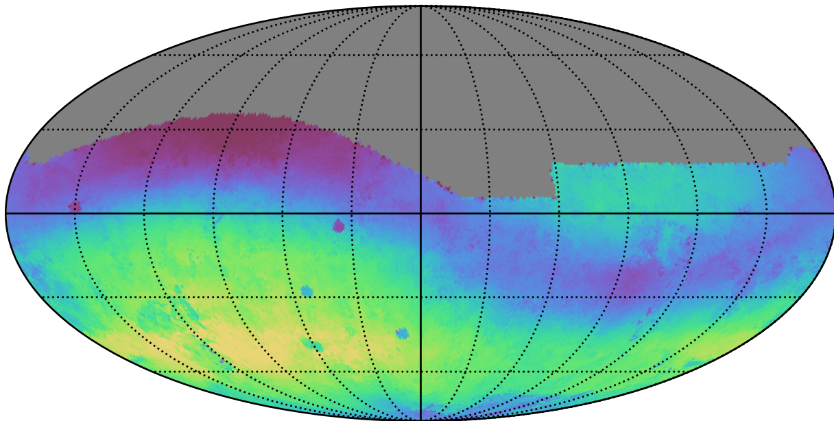
extra_ss_neo3_v3.4_10yrs All sky g band: Median skyBrightness
