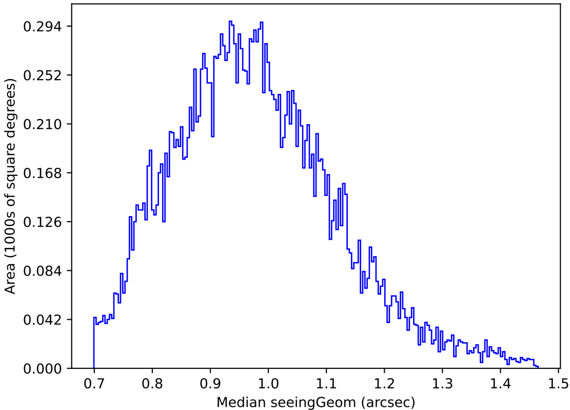
extra_ss_neo3_v3.4_10yrs Yr 1 u band: Median seeingGeom
