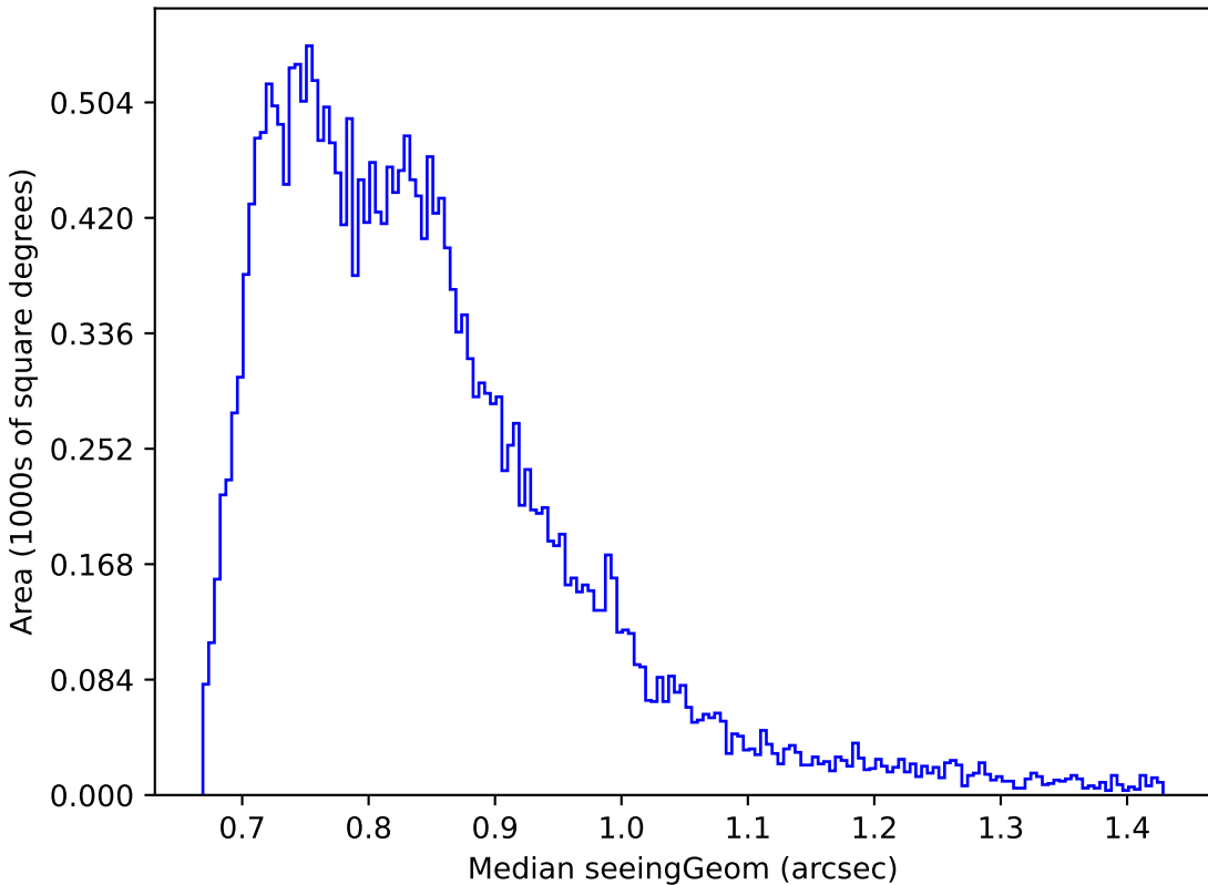
extra_ss_neo3_v3.4_10yrs Yr 1 i band: Median seeingGeom
