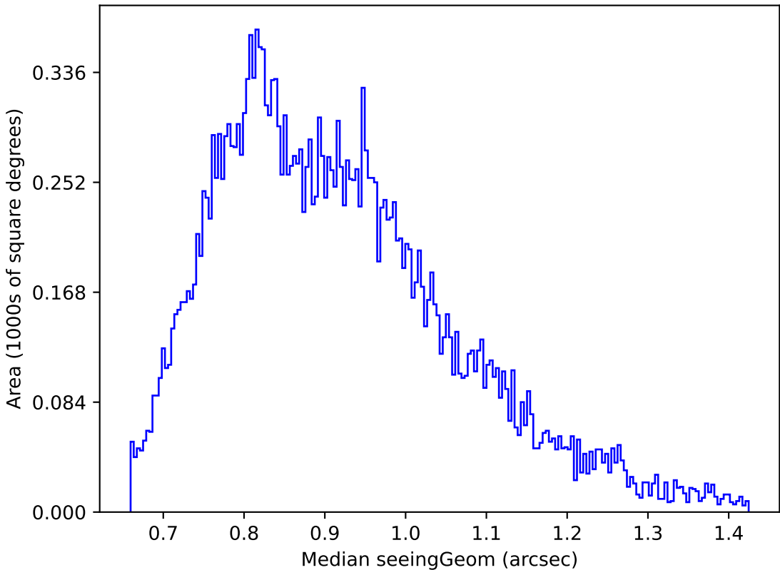
extra_ss_neo3_v3.4_10yrs Yr 1 g band: Median seeingGeom
