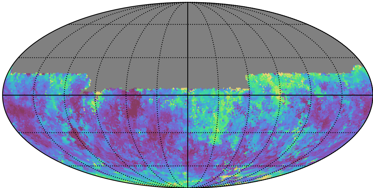
extra_ss_neo3_v3.4_10yrs Yr 1 y band: Median seeingEff
