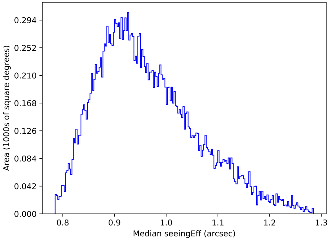
extra_ss_neo3_v3.4_10yrs Yr 1 y band: Median seeingEff
